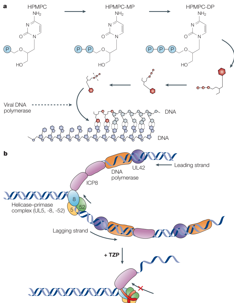
Figure 3 | The mechanism of action of cidofovir and HSV helicase-primase complex inhibitors. a | The mechanism of antiviral action of cidofovir (HPMPDC). As an acyclic nucleoside phosphonate, cidofovir is not dependent on activation by a virus-encoded enzyme for activity. Two phosphorylations are required for activity. Reproduced with permission from REF. 1 © Nature Rev. Drug Discov. (2002) Nature Publishing Group. b | The mechanism of inhibition of DNA synthesis by HSV helicase-primase complex inhibitors. The helicase-primase complex comprises the viral gene products UL5, -8 and -52. This complex unwinds HSV DNA at the replication fork and primes DNA synthesis at both the lagging and the leading strands. The single-stranded-DNA-binding protein ICP8 binds to single-stranded template DNA. HSV DNA polymerase and its accessory protein UL42, promote leading- and lagging-strand DNA synthesis. The TZIP (amino-thiazolyphenyl)-containing compounds (red band) enhance binding of the UL5 and UL52 subunits of the helicase-primase complex to both the leading- and the lagging-strand DNA, resulting in inhibition of helicase activity, primase activity and viral DNA synthesis. Modified with permission from REF. 15 © Nature Medicine (2002) Nature Publishing Group.
